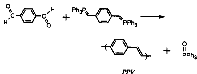
Figure 1. Wittig route to PPV.
