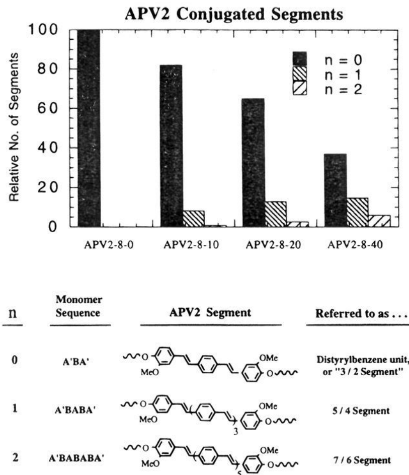
Figure 6. Calculated densities of various phenylene vinylene segment lengths ( n = 0, 1, \text{ or } 2 ) within a random APV copolymer chain containing 100 units (AB or A'B). The relative amounts of phenylene vinylene segments are calculated for each of the four cases where the mole fraction of A is 0, 0.1, 0.2, or 0.4—the "PPV content" in the copolymer backbone.
