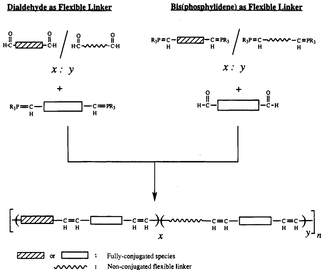
Figure 2. Wittig routes to aliphatic phenylene vinylene copolymers.
